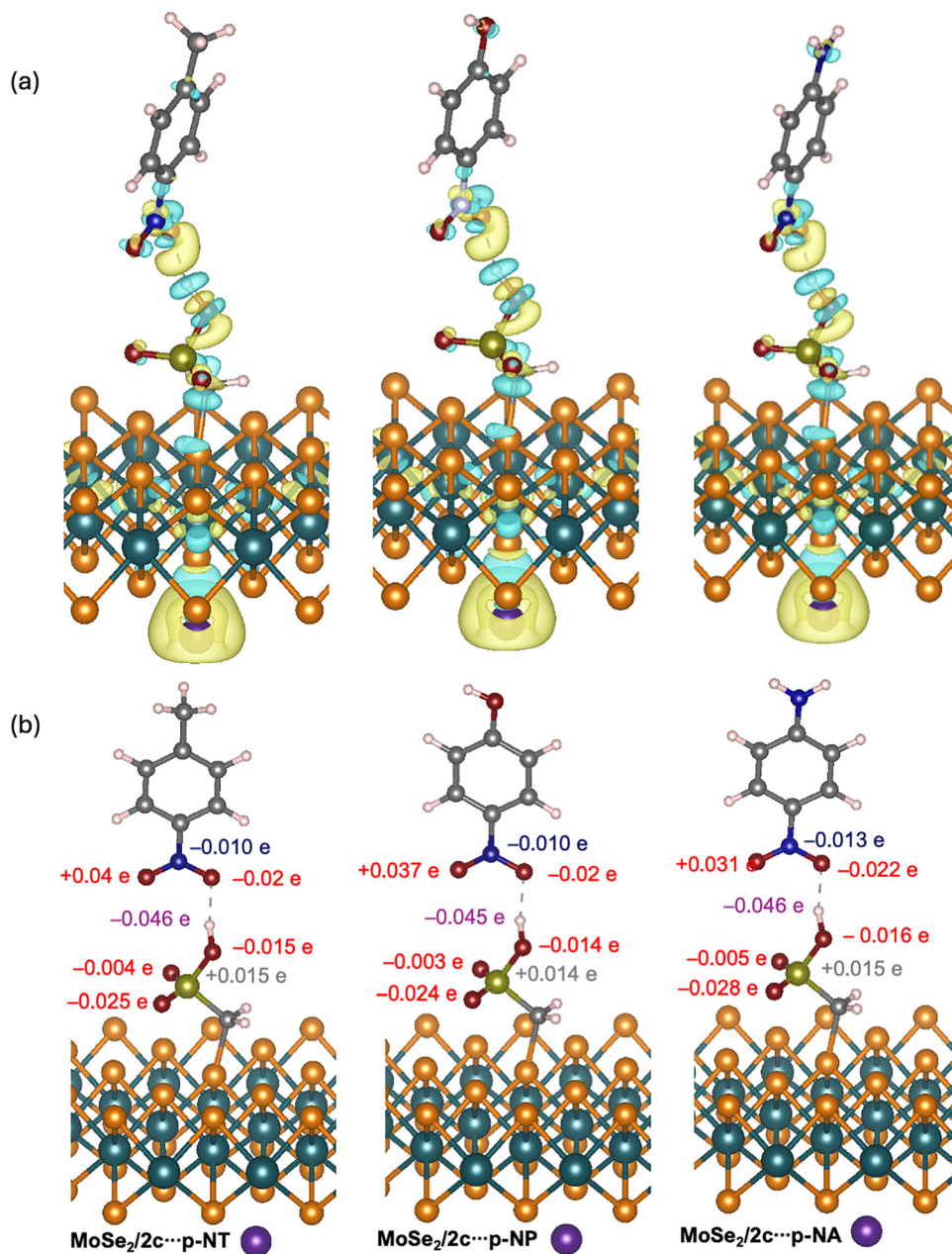
Fig. 4 (a) Electronic density differences and (b) Löwdin partial charges for \text{MoSe}_2/2c interacting with p -NT, p -NP, and p -NA target molecules. The charge density differences were plotted at a density isovalue of 2.5 \times 10^{-3} e \text{ Bohr}^{-3} .
