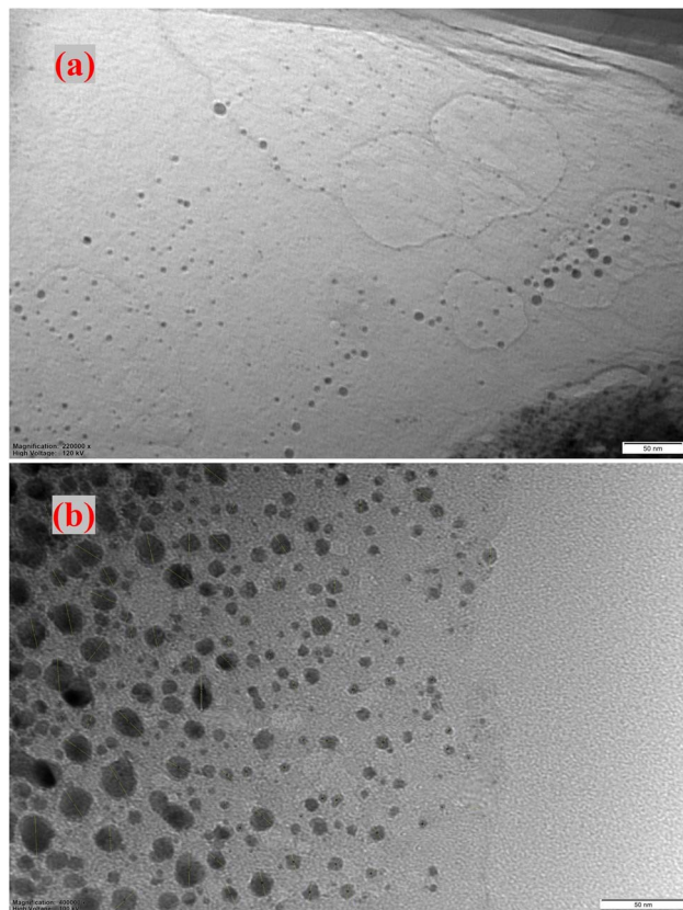
Fig. 3 TEM image micrographs of uncapped FeCoNiCuPt nanoparticles taken (a) after 1 hour and (b) after 10 days of washing out the isolating medium and storing in ethanol at -20 °C.
