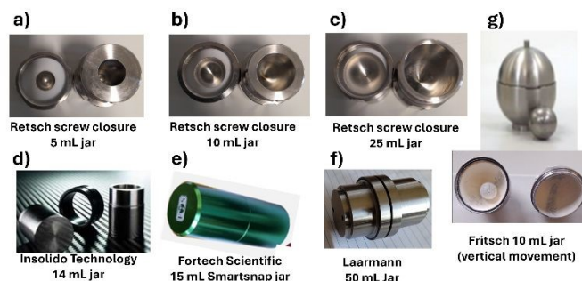
Figure 3 Commercially available jars used for vibrational ball milling. The internal shape of the top and bottom caps are hemispheres, connected through a cylindrical section. a) to f) used under horizontal vibratory motion using ball mills depicted in Figure 2b). The milling jar in g) is used for vertical motion using ball mills depicted in Figure 2c).
