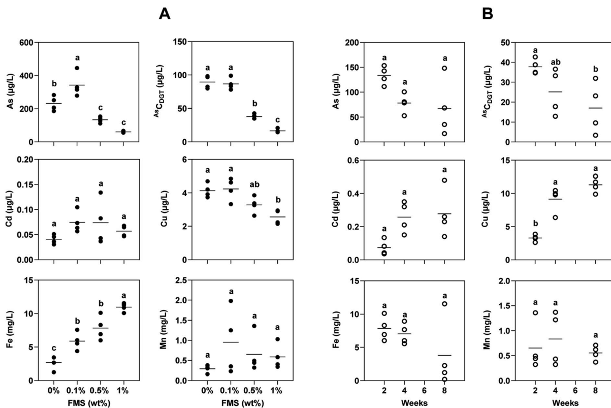
Fig. 4 Effect of FMS on element concentration in soil pore-water ( C_{sol} ) and DGT measured As ( ^{55}C_{DGT} ) (Mean, n = 4 ). (GLM, post hoc analysis was carried out using Tukey Pairwise Comparisons). Different letters above each bar represent significant differences between treatments ( P < 0.05 ). (A): Dose. (B): Time.
