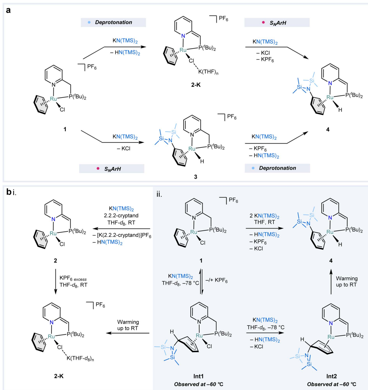
Fig. 4 Plausible mechanisms and mechanistic investigations of the S_N\text{ArH} reaction with \text{KN}(\text{TMS})_2 . (a) Plausible mechanistic pathway involving first deprotonation of the methylene linker of the {}^t\text{BuPN} ligand followed by nucleophilic aromatic substitution of a hydride (top path) and a pathway wherein the S_N\text{ArH} precedes the deprotonation of the {}^t\text{BuPN} ligand (bottom path). (b) Mechanistic NMR experiments at RT (i) and -60\text{ }^{\circ}\text{C} (ii) featuring the structures of two kinetically-trapped metal-stabilized Jackson–Meisenheimer intermediates Int1 and Int2 .
