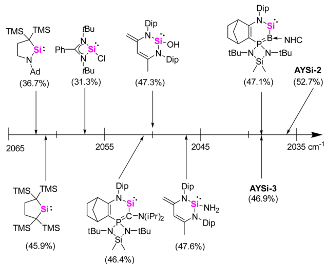
Fig. 4 Comparison of the TEP values for various silylenes determined by asymmetric CO stretching frequency of \sigma -Ni(CO) 3 in toluene at room temperature. 26,31 % V_{\text{bur}} is given in parentheses.
