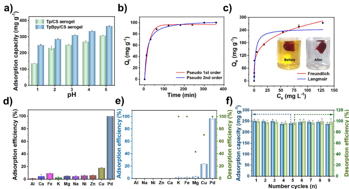
Fig. 2 (a) Effect of pH on adsorption of Pd(II) (conditions: adsorbent dosage: 5 mg; V = 10.0 mL; C_{Pd} = 250 mg L -1 ; temperature: 25 °C; time: 24 h); (b) the pseudo 1st order and pseudo 2nd order kinetics models of Pd(II) adsorption by TpBpy/CS aerogel; (c) the Freundlich and Langmuir model of Pd(II) adsorption by TpBpy/CS aerogel (the inserted photograph shows the color change of the solution before and after the adsorption of Pd(II) by TpBpy/CS aerogel); (d) adsorption selectivity (conditions: adsorbent dosage: 5 mg; V = 10.0 mL; C_{Pd} = 10 mg L -1 ; C_{other} = 1000 mg L -1 ; temperature: 25 °C; pH = 1; time: 24 h); (e) adsorption and desorption efficiency of TpBpy/CS aerogel in actual metallurgical wastewater; (f) reusability of the TpBpy/CS aerogel.
