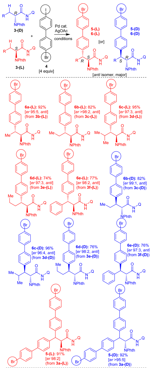
Scheme 4 Construction of enantioenriched amino acid derivatives possessing a 4-bromobiphenyl moiety via the Pd(II)-catalyzed \beta -C-H arylation. Conditions: 3-D or 3-L (0.25–4.6 mmol), Pd(OAc) 2 (10 mol%), AgOAc (2.5 equiv.), toluene (3 mL), 110 °C, 48 h, sealed tube (purged with N 2 ). Products 6-L (or) 6-D were obtained from their corresponding carboxamides of 2-aminobutyric acid 3b-L , norvaline 3c-L/D , leucine 3d-L/D , norleucine 3e-L/D , phenylalanine 3f-L/D and 2-aminooctanoic acid 3g-DL linked with 8-aminoquinoline directing group. Products 5-L (or) 5-D were obtained from their corresponding carboxamides of alanine 3a-L/D linked with 8-aminoquinoline directing group.
