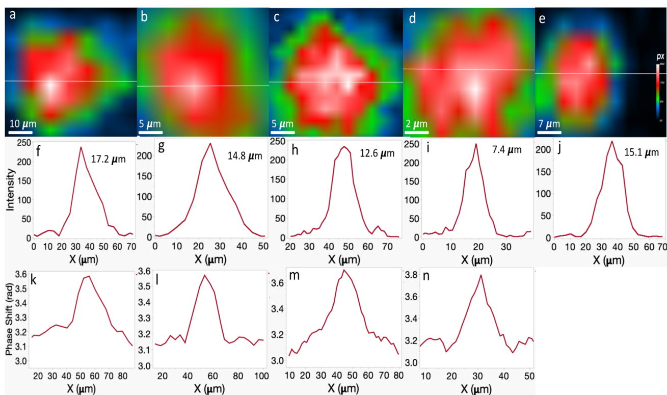
Fig. 4 Reconstruction of airborne BC particles using AI-Nano-DIHM: (a–e) Intensity reconstruction of distinct BC particles captured in the air phase. (f–j) Intensity profiles through the particles' crosscuts, (k–n) show the phase profiles through the particles' crosscuts. Note that the phase profile of particle (e) could not be detected. Results confirm the AI-Nano-DIHM's ability to resolve airborne BC particles with submicron–micron resolution in real time.
