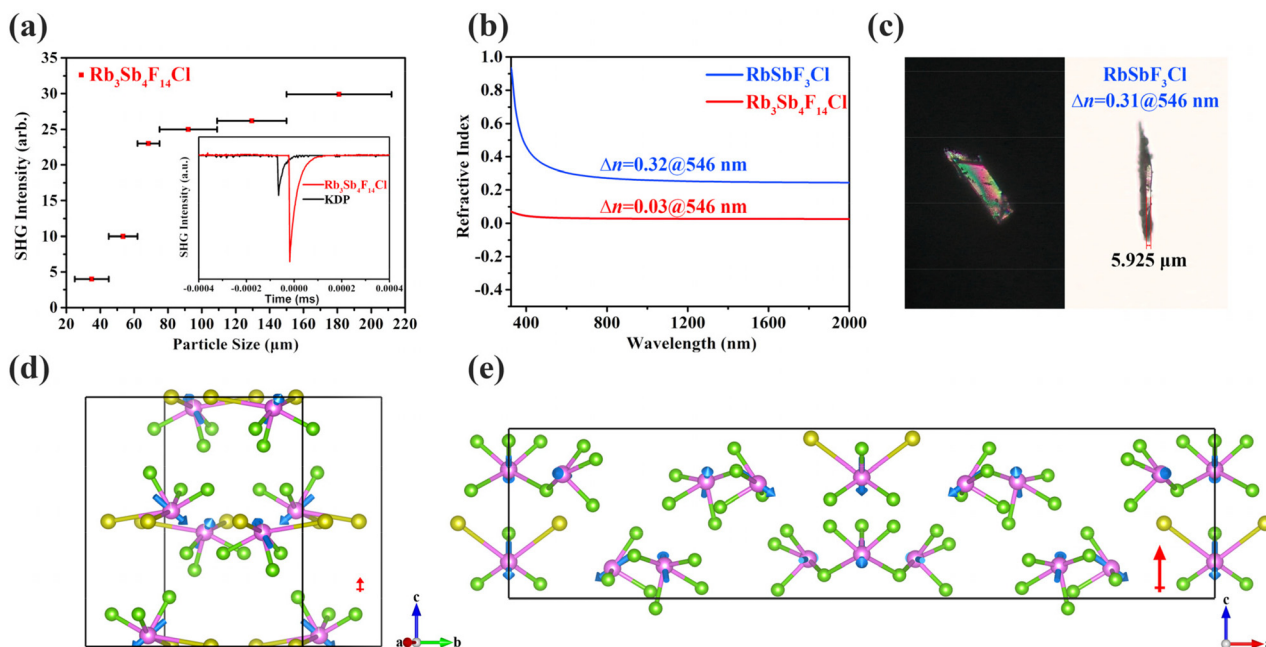
Fig. 3 (a) The phase-matching curve for Rb 3 Sb 4 F 14 Cl. Inset: SHG intensity with KDP as the reference (150–212 \mu\text{m} ). (b) Calculated birefringence for RbSbF 3 Cl and Rb 3 Sb 4 F 14 Cl. (c) The experimental birefringence of RbSbF 3 Cl. (d) The orientations of the lone pair of electrons in the unit cell of RbSbF 3 Cl. (e) The orientations of the lone pair of electrons on Sb 3+ within a single cell in Rb 3 Sb 4 F 14 Cl. The direction of the overall dipole moments is highlighted by a red arrow.
