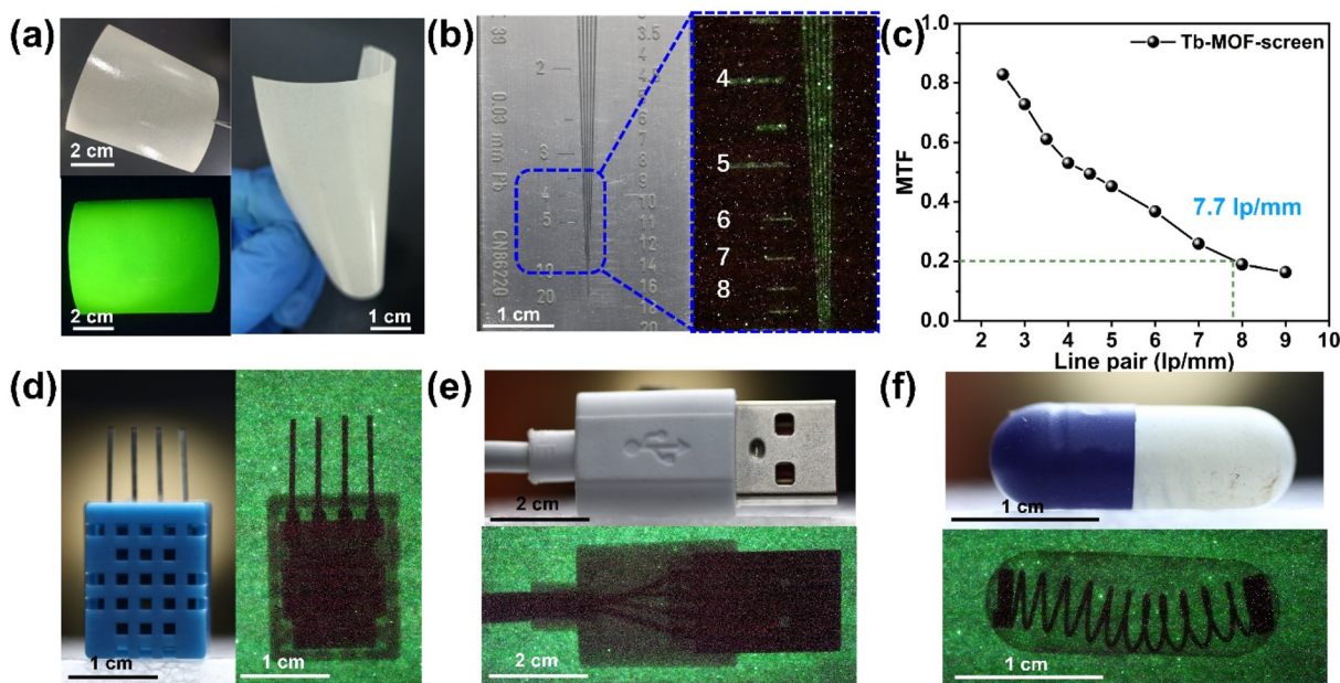
Fig. 4 (a) The photographs of the flexible Tb-MOF-screen . (b) Profile displays (left) and X-ray images (right) of the standard line pair card. (c) MTF of the X-ray image based on the standard line pair card. The real pictures and X-ray radiographs of the electronic component (d), the USB connector (e), and the capsule (f).
