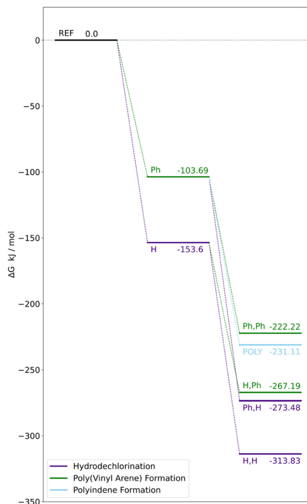
Fig. 4 Computationally predicted free energy changes (kJ mol -1 at 298 K) associated with hydrodechlorination, Friedel–Crafts alkylation, polyindene formation and combinations of these reactions for model PVC systems. The states are colored and labelled based on the reaction step: 'Ph' indicates benzene addition, 'H' to hydride addition, and 'POLY' to polyindene formation.
