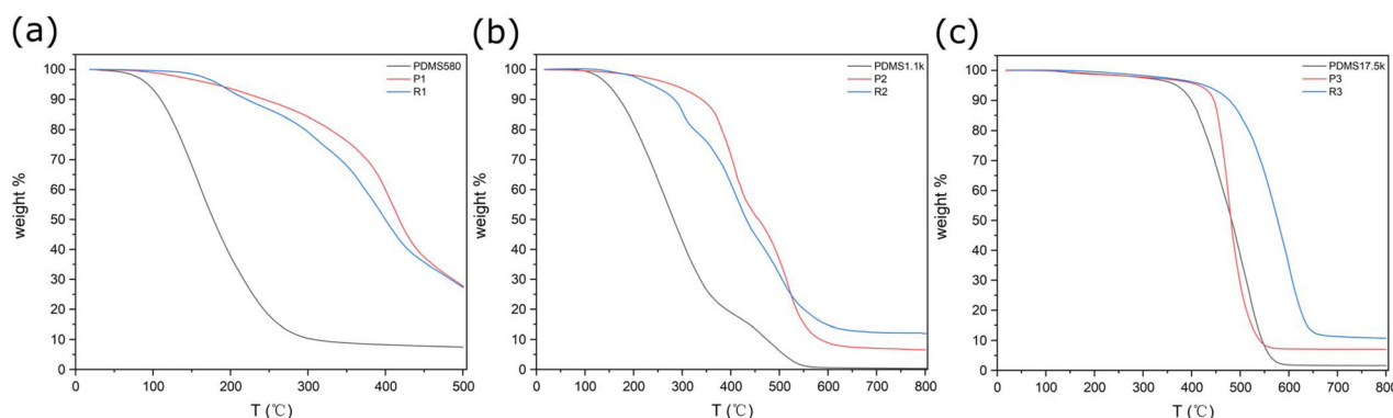
Fig. 2 TGA curves of (a) PDMS-580, P1 , and R1 ; (b) PDMS-1.1k, P2 , and R2 ; (c) PDMS-17.5k, P3 , and R3 at the heating rate of 10\text{ °C min}^{-1} under flowing nitrogen.
