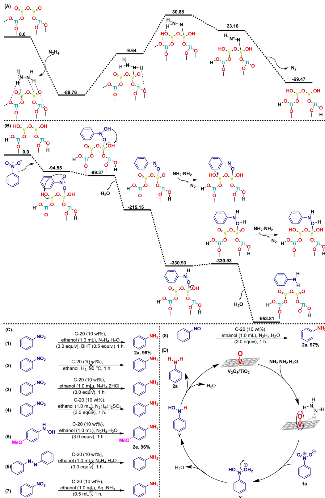
Fig. 7 (A) Reaction energy profile of dehydrogenation of N_2H_4 over the V_2O_5/TiO_2 (001) surface (reaction energies are labelled in \text{kJ mol}^{-1} ), (B) reaction energy profile of nitrobenzene reduction to aniline over hydrogenated V_2O_5/TiO_2 (001) (reaction energies are labelled in \text{kJ mol}^{-1} ), (C) control experiments and (D) plausible mechanism.
