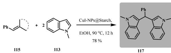
Scheme 51 Copper nanoparticle catalysed synthesis of bisindolylmethane (Suresh et al. ).
