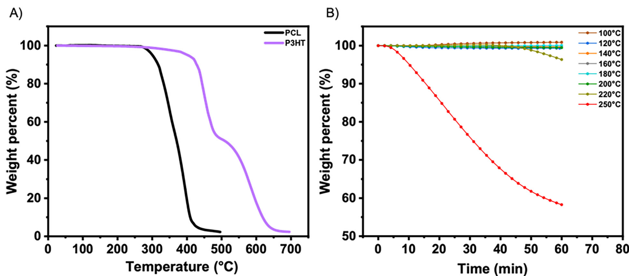
Fig. 2 (A) Thermogravimetric analyses of PCL and P3HT. (B) Isothermal thermogravimetric analyses under air atmosphere of PCL at different temperatures for 60 min.
