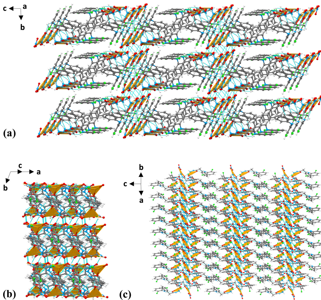
Fig. 6 (a) Supramolecular multilayer infinite 3D framework mediated by multiple intermolecular \text{N-H}\cdots\text{O}/\text{C-H}\cdots\text{O} hydrogen bond linkages (turquoise dashed lines) in complex 1 , (b) twisting candy wrap-shaped 3D perspective layered structure of complex 1 , layers added towards the b -axis and interconnected through intermolecular hydrogen bonds from a/c packing, and (c) birds flying-shaped 3D perspective layered structure of complex 1 .
