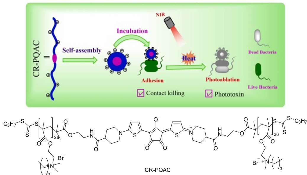
Fig. 14 Molecular structure of CR-PQAC and its antibacterial mechanisms. Reproduced with permission from ref. 111 (modified). Copyright 2024, Elsevier.
