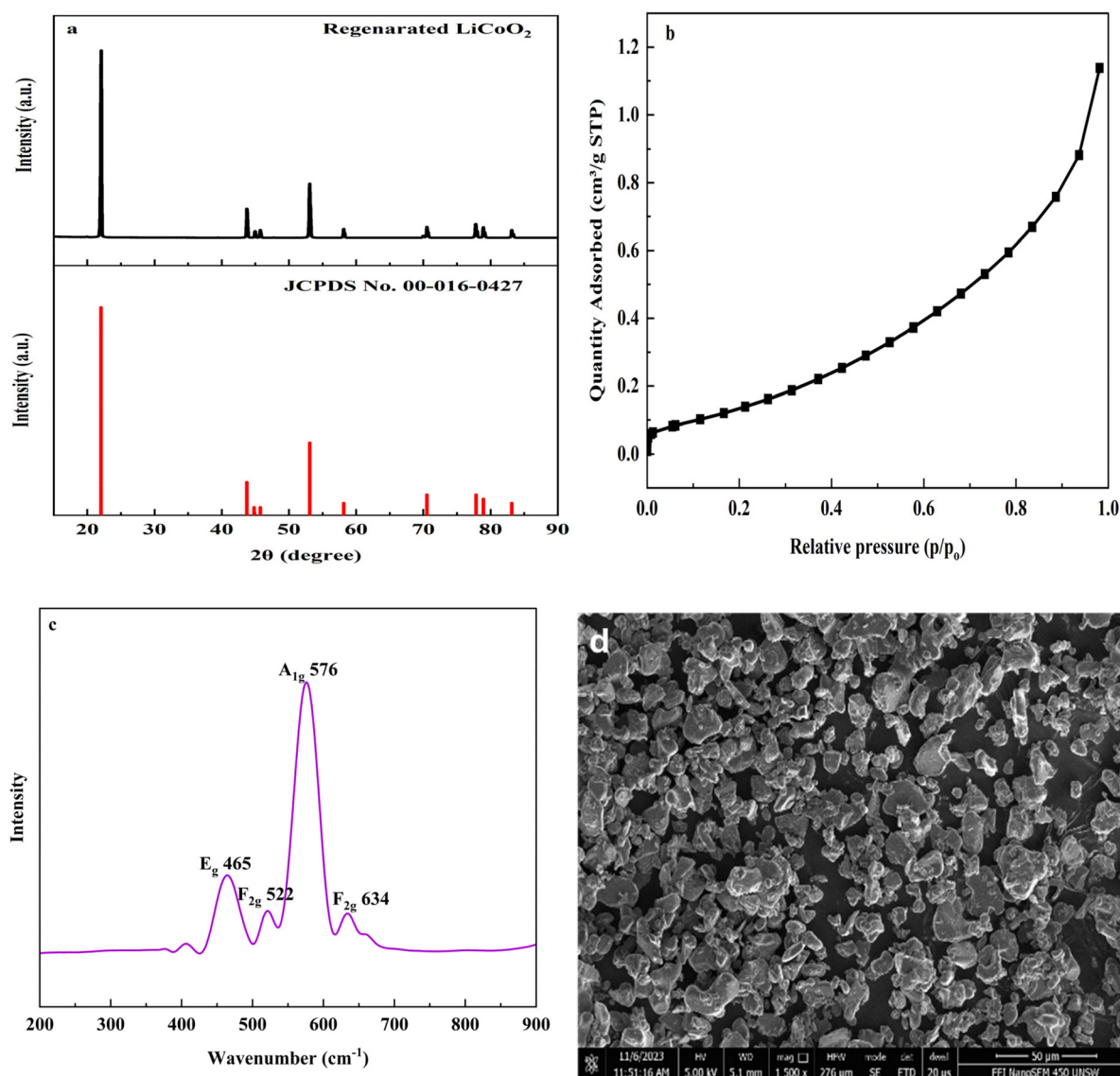
Fig. 9 Characterization of regenerated \text{LiCoO}_2 : (a) XRD pattern; (b) BET surface area; (c) Raman spectra; (d) SEM.
