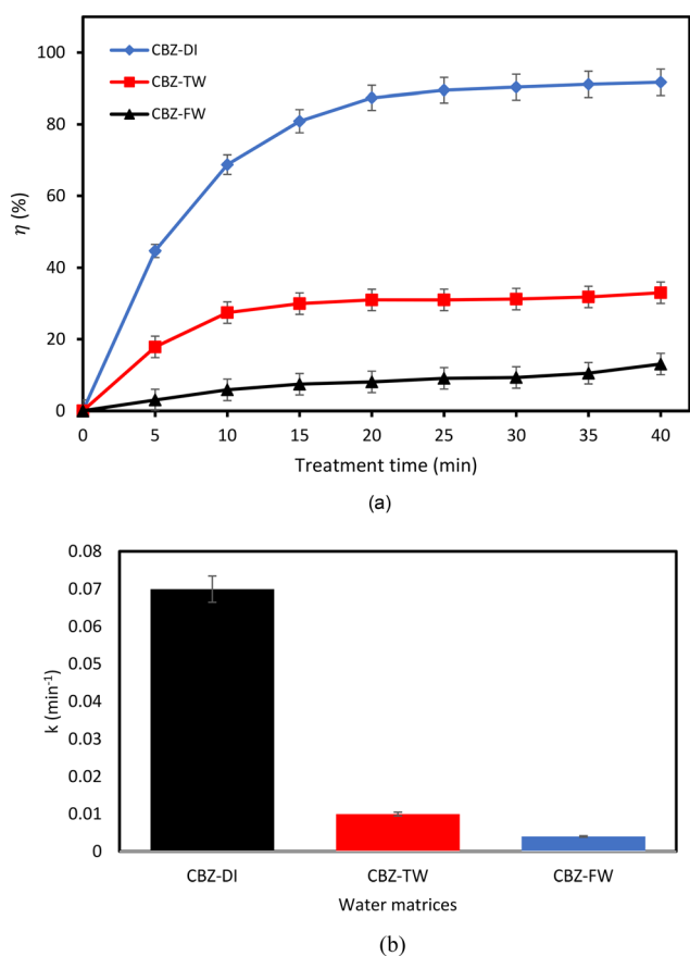
Fig. 13 (a) Effect of water matrices on degradation efficiency of CBZ. (b) Effect of water matrices on reaction rate for CBZ degradation (experimental conditions: CBZ initial concentration 10 \text{ mg L}^{-1} ; voltage 6 kV; frequency 20 kHz).
