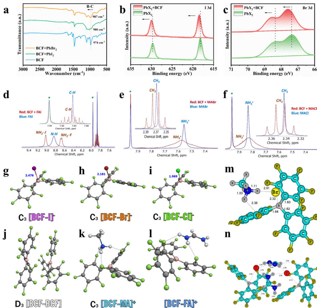
Fig. 1 FTIR spectra of (a) BCF and BCF + \text{PbX}_2 mixture. XPS spectra of (b) I 3d and (c) Br 3d for \text{PbX}_2 and \text{PbX}_2 + \text{BCF} films, respectively. The evolution of the ^1\text{H} NMR spectra of FAI (d), MABr (e) and MACl (f) upon interaction with BCF. The geometrical configuration of the [\text{BCF}-\text{I}]^- (g), [\text{BCF}-\text{Br}]^- (h), [\text{BCF}-\text{Cl}]^- (i) anionic complexes. The [\text{BCF}-\text{BCF}] neutral dimer (j), and the [\text{BCF}-\text{MA}]^+ (k) and [\text{BCF}-\text{FA}]^+ (l) cationic complexes, where symmetry is present it is listed before the complex name. The computed minimal-energy molecular structures of the MABr + BCF (1:1, m) and FAI + BCF (2:2, n) complexes. Short contacts are shown in the figures.
