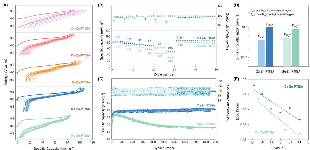
Fig. 4 Divalent cation storage performances of the DI-M-PTtSA materials. (A) Galvanostatic voltage-capacity profiles for Mg/Ca/Sr/Ba/Zn-Zn-PTtSA acquired at a rate of C/10 (1C being equivalent of 100/97/89/82/93 mA g -1 , respectively). (B) Capacity retention at different cycling rates for Ca-ion and Mg-ion electrodes (1C is equal to 100 mA g -1 for Mg-Zn-PTtSA and 97 mA g -1 for Ca-Zn-PTtSA). (C) Long-term cycling performances of Mg/Ca-Zn-PTtSA cells cycled at a current density of 100 mA g -1 (or 1C rate). (D) Diffusion coefficients and (E) electrical conductivity of Ca- and Mg-Zn-PTtSA CPs. The electrolyte formulations used in (A) were 0.5 M Ca (TFSI) 2 DME for Ca 2+ , 0.1 M Mg(ClO 4 ) 2 PC for Mg 2+ , 0.5 M Sr(ClO 4 ) 2 ACN for Sr 2+ , 0.5 M Ba(ClO 4 ) 2 ACN for Ba 2+ and 0.5 M Zn(TFSI) 2 DME for Zn 2+ storage.
