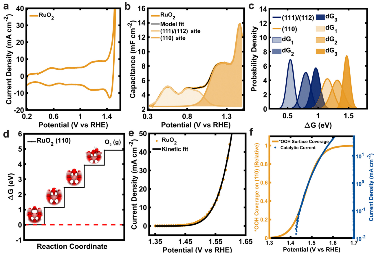
Fig. 2 Electrodesorption and kinetic analysis of \text{RuO}_2 electrocatalyst synthesized at 700^\circ\text{C} . (a) Cyclic voltammogram scanned at 1\text{ V s}^{-1} . (b) Comparison of electrodesorption model fits of (111)/(112) and (110) sites to electrodesorption profile derived from (a). (c) Distributions of reaction energies for the first three electron-transfer steps involved in the OER. (d) Free energy diagram constructed from electrodesorption analysis. (e) Comparison between steady-state current density and kinetic model fit. (f) Surface coverage of ^*\text{OOH} species on (110) site and catalytic current density versus potential.
