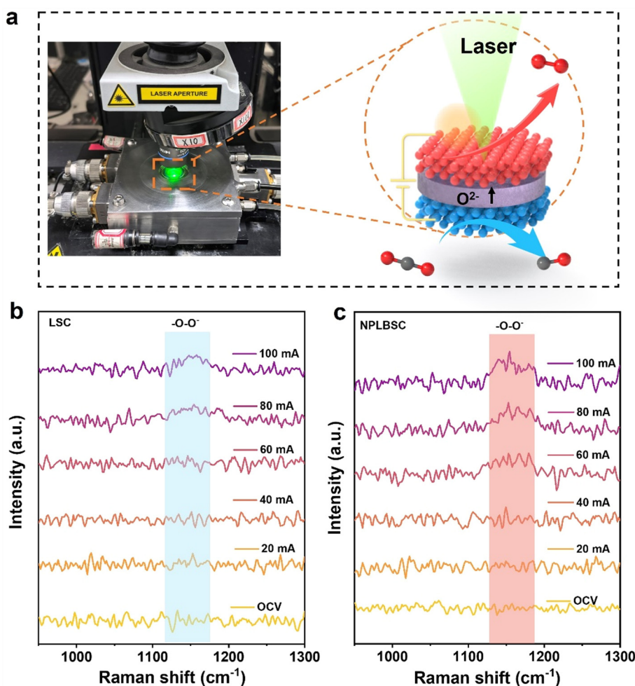
Fig. 4 In situ Raman spectroscopy tests. (a) Picture and schematics of the in situ Raman spectroscopy cells. In situ Raman spectra of (b) LSC and (c) NPLBSC at 600 °C, respectively.
