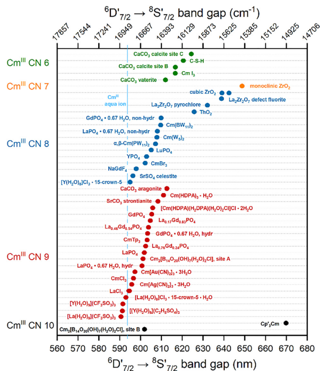
Fig. 9 \text{Cm}^{\text{III}} emission peak maxima of selected Cm-doped or Cm-based crystalline solid phases, organized by coordination number. The pale blue vertical dashed line indicates the emission maximum of the \text{Cm}^{\text{III}} aqua ion at 593.8 nm, serving as a reference point for bathochromic or hypsochromic shifts across different coordination environments. Peak positions and corresponding references for all compounds are discussed in Section 3 or Section 6, with the exception of: \text{LaCl}_3 , 81 ( \text{CmCl}_3 , \text{CmBr}_3 , \text{CmI}_3 ), 74 ( \text{YPO}_4 , \text{LuPO}_4 ), 82 and \text{ThO}_2 . 83
