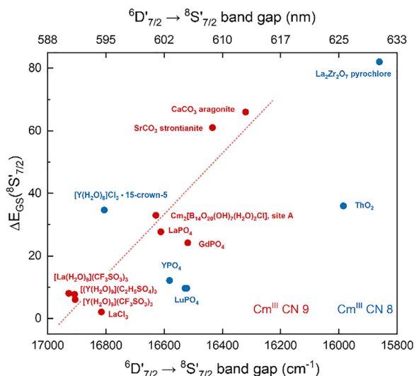
Fig. 10 Correlation between ground-state splitting \Delta E_{GS}(^8S'_{7/2}) and emission peak maximum ( ^6D'_{7/2} \rightarrow ^8S'_{7/2} band gap energy) for \text{Cm}^{III} in selected solid phases with eight- and nine-fold coordination.
