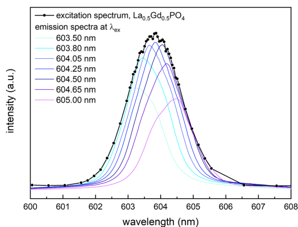
Fig. 6 Luminescence line narrowing can be observed following direct excitation of \text{Cm}^{\text{III}} in solid phases lacking long-range order (e.g., amorphous materials), or in systems with random cation distribution, such as disordered (statistical) solid solutions. \lambda_{\text{ex}} refers to excitation wavelength used for the collection of the emission spectra (colored traces). Adapted in part from ref. 51. Copyright 2018 American Chemical Society.
