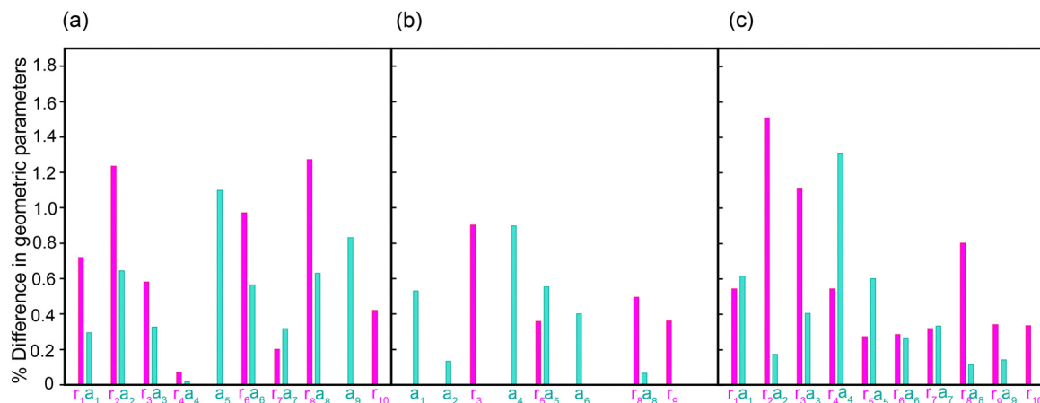
Fig. 6 Deviations in the structural parameters of (a) Q_{C1,75}^{21} and (b) Q_{C1,67}^{21} in relation to the FC geometry of PM650. (c) Deviations in the structural parameters of Q_{C1,96}^{21} in relation to the FC geometry of PM597.
