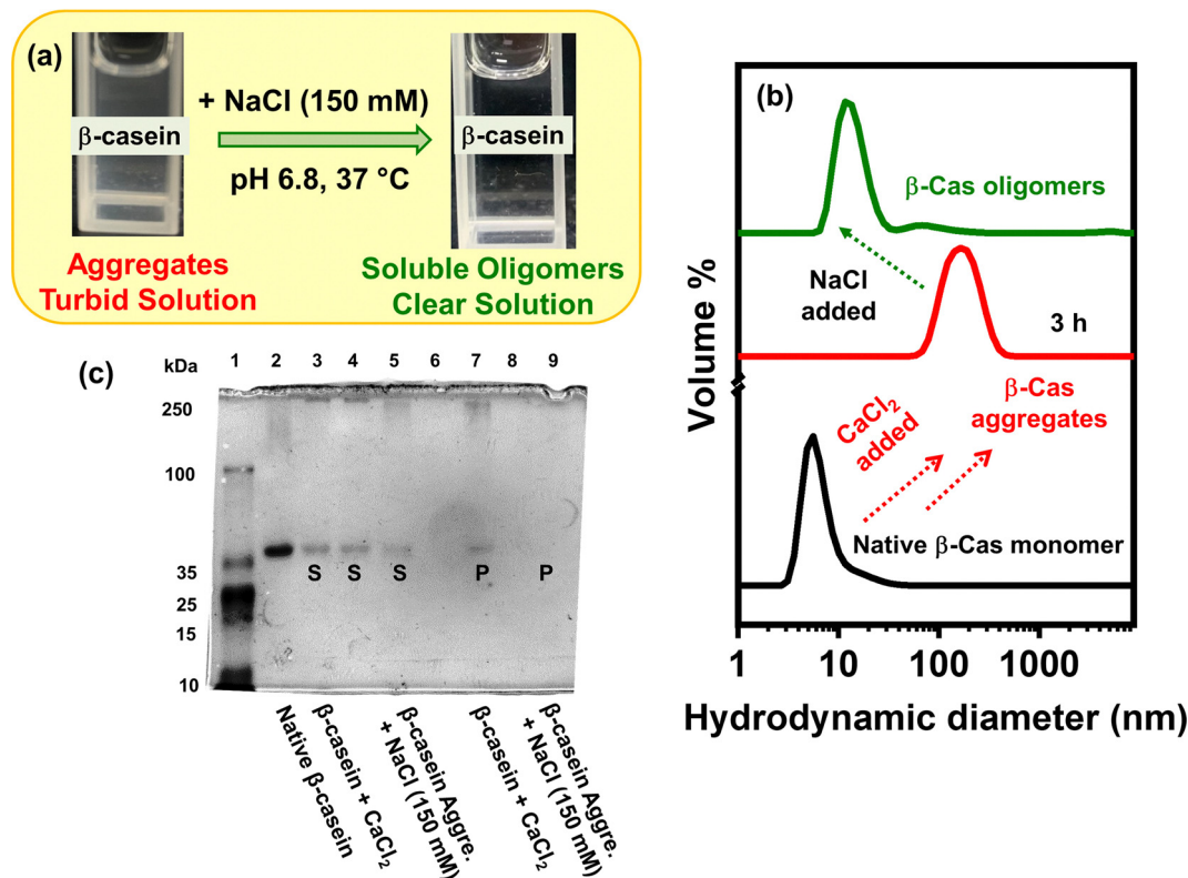
Fig. 1 Disruption of \text{Ca}^{2+} -induced \beta -casein aggregates formed at pH 6.8, 37\text{ }^{\circ}\text{C} upon the addition of 150 mM sodium chloride (NaCl) to the preformed aggregates. (a) Disappearance of the solution turbidity, observed visually, resulting in a clear solution. (b) Hydrodynamic diameter of the native \beta -casein (black) and \beta -casein aggregates (red) formed after 3 h of incubation in the presence of 2.5 mM \text{CaCl}_2 , pH 6.8, 37\text{ }^{\circ}\text{C} , monitored using dynamic light scattering (DLS), depicted by a stack-plot representation. A significant reduction in the hydrodynamic diameter of \beta -casein aggregates, upon the addition of 150 mM NaCl (shown by a green dashed arrow), indicates dissolution of the aggregates leading to aggregation-incompetent, soluble oligomers (green). (c) Native-PAGE analyses of native \beta -casein monomer (lane 2), \text{Ca}^{2+} -induced \beta -casein aggregates formed at \sim 37\text{ }^{\circ}\text{C} (lanes 3 and 7) and upon the addition of 150 mM NaCl (post-addition approach) into the preformed \beta -casein aggregates after 3 h of incubation (lanes 5 and 9) (S: supernatant, P: pellet).
