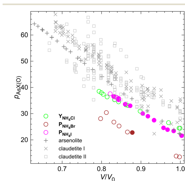
Fig. 4 Penetration indices of As \cdots X and As \cdots O secondary bonds in the studied intercalates and As _2 O _3 polymorphs plotted as a function of V/V_0 unit-cell volume ratio. Data for arsenic(III) oxide polymorphs are taken from ref. 34–36.
