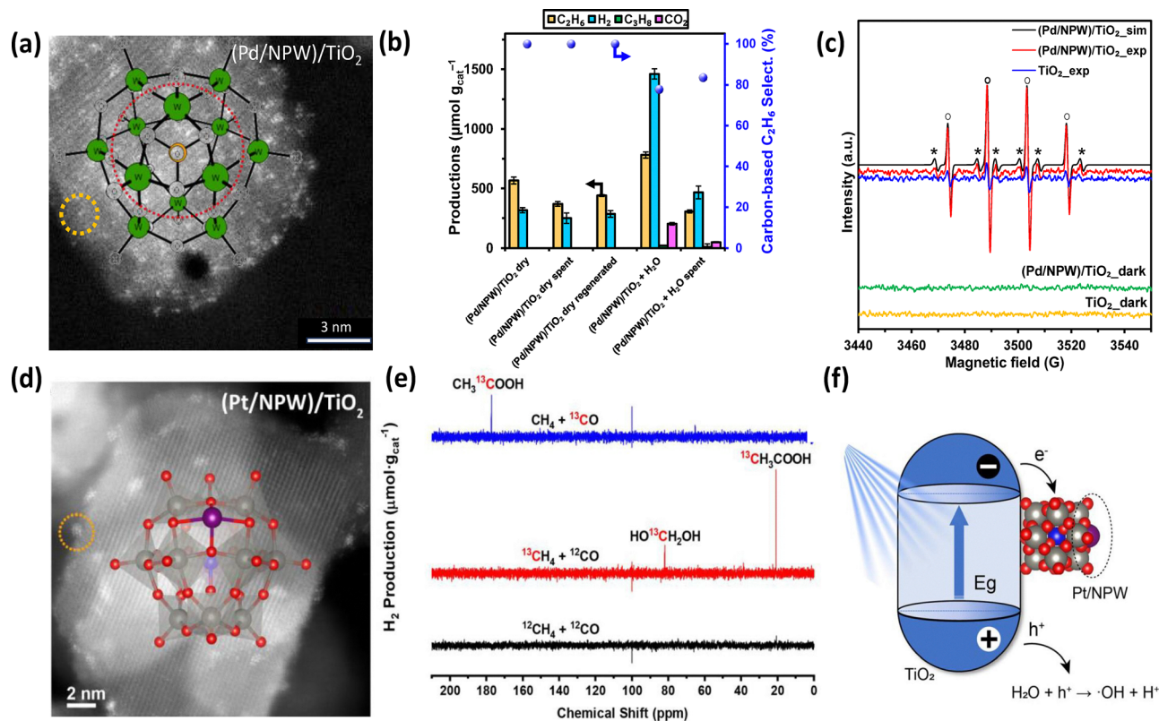
Fig. 6 (a) STEM-HAADF images of (Pd/NPW)/ \text{TiO}_2 . Color code: O – white, P – orange, W – green. (b) Methane photocatalytic coupling on (Pd/NPW)/ \text{TiO}_2 nanocomposites in dry and aqueous environments. (c) EPR spectra of DMPO spin trapping of (Pd/NPW)/ \text{TiO}_2 and \text{TiO}_2 under methane. *Signals of \text{DMPO}/\cdot\text{CH}_3 , \cdot\text{OH} signals of \text{DMPO}/\cdot\text{OH} . 37 Reproduced from ref. 37 with permission from Elsevier, copyright 2024. (d) Atomic-resolved HAADF-STEM image of Pt/NPW/ \text{TiO}_2 (3 : 10). The inset image represents the monomer of Keggin-structured NPW with isolated Pt atoms anchored at the 4-fold hollow site of W–O–W, color code: red (oxygen), gray (tungsten), blue (phosphorus), purple (platinum). (e) ^{13}\text{C} NMR spectra of liquid products of (Pt/NPW)/ \text{TiO}_2 (3 : 5) with ^{12}\text{CH}_4 + ^{12}\text{CO} , ^{13}\text{CH}_4 + ^{12}\text{CO} , and ^{12}\text{CH}_4 + ^{13}\text{CO} . (f) Scheme of the generation of photoexcited charge carriers by Pt/NPW. 104 Reproduced from ref. 104 with permission from American Chemical Society, copyright 2023.
