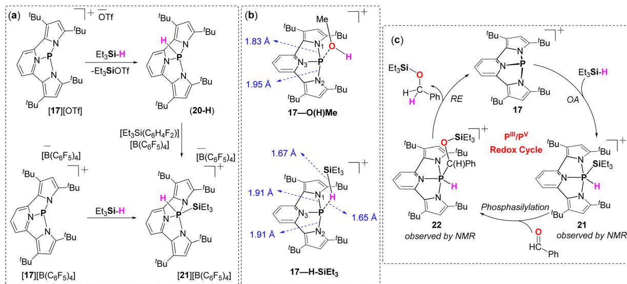
Fig. 10 (a) Si–H bond activation by [17][OTf] and [17][B(C_6F_5)_4] ; (b) DFT optimized structure of 17-O(H)Me , 17-H-SiEt 3 and their bond lengths around P atom; (c) hydrosilylation reaction catalyzed by [17][B(C_6F_5)_4] .
