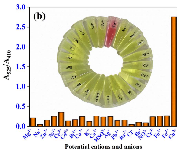
Fig. 1 UV-vis absorption spectral profile (a) for RME (10 \mu M) and after the addition of \text{Cu}^{2+} ions (100 \mu M) and the inset represents the RME before (i) and after (ii) the addition of \text{Cu}^{2+} ions into the receptor RME in DMF/water (1 : 2, v/v) medium. Bar graph (b) of RME with the addition of different metal cations and anions and the inset visualizes the notable color changes of RME solution containing different metal cations and anions in DMF/water (1 : 2, v/v) medium.
