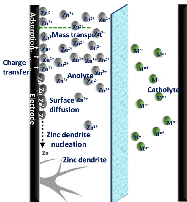
Fig. 5 Schematic representation of Zn-dendrite formation at the anode.
