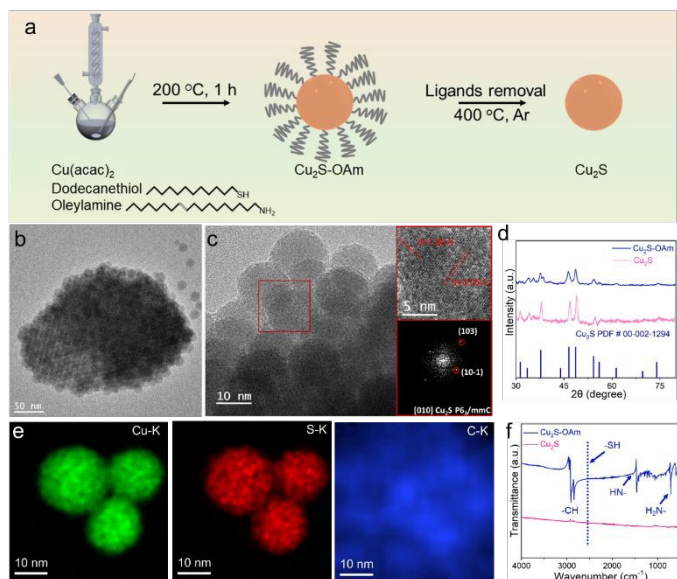
Figure 1. (a) Scheme of the procedure used to prepare \text{Cu}_2\text{S} -OAm and \text{Cu}_2\text{S} . (b) TEM and (c) HRTEM images and indexed power spectrum of \text{Cu}_2\text{S} -OAm NPs. From the crystalline domain, the \text{Cu}_2\text{S} lattice fringe distances were measured to be 0.1902 nm, 0.3057 nm, at 80.46^\circ which is interpreted as the hexagonal \text{Cu}_2\text{S} phase, visualized along its [101] zone axis. (d) STEM-EDS chemical composition maps of \text{Cu}_2\text{S} -OAm NPs; (e) XRD patterns of \text{Cu}_2\text{S} and \text{Cu}_2\text{S} -OAm. (f) FT-IR spectra of \text{Cu}_2\text{S} and \text{Cu}_2\text{S} -OAm.
