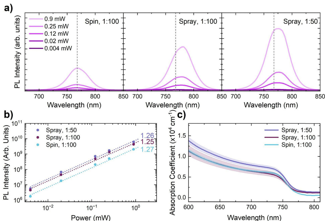
Fig. 3 Optoelectronic properties of Cs 0.05 FA 0.81 MA 0.14 PbI 2.55 Br 0.45 thin films on Al 2 O 3 treated Me-4PACz on indium tin oxide (ITO) glass. Ratios represent dilution of nanoparticles: isopropanol. (a) Intensity dependent steady-state photoluminescence spectra, the integrated area under the peak was then used to calculate (b) the ideality factor, and (c) the absorption coefficient as determined through ultraviolet-visible spectroscopy measurements. The shaded area represents the uncertainty in these measurements.
