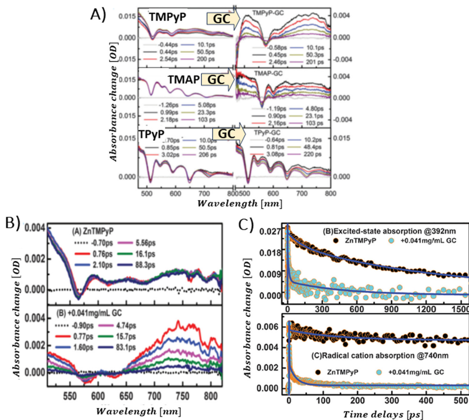
Fig. 17 (A) TAS recorded after 425 nm pulsed laser excitation (120 fs) for TPpP, TMAP and TMPyP prior to (left) and following (right) the introduction of GC. Reprinted with permission from ref. 93. Copyright 2014, Royal Society of Chemistry. (B) TAS observed at different time delays for free ZnTMPyP and in the presence of GC (0.04 mg mL -1 ). (C) Normalized transient absorption time profiles taken at 392 nm and 740 nm for ZnTMPyP and ZnTMPyP/GC. Adapted from ref. 106 with permission from the PCCP Owner Societies.
