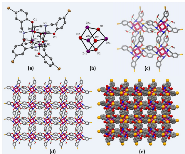
Fig. 1 (a) Ortep view of Zn(II) cubane, (b) framework of the Zn 4 O 4 cubane cage, (c) wireframe representation of interactions between crystallized cubane units, (d) crystal packing of Zn(II) cubane showing 2-D sheet-like view, (e) space-fill representation of Zn(II) cubane (for non-hydrogen atoms, the radius of hydrogen atoms was eliminated for clarity).
