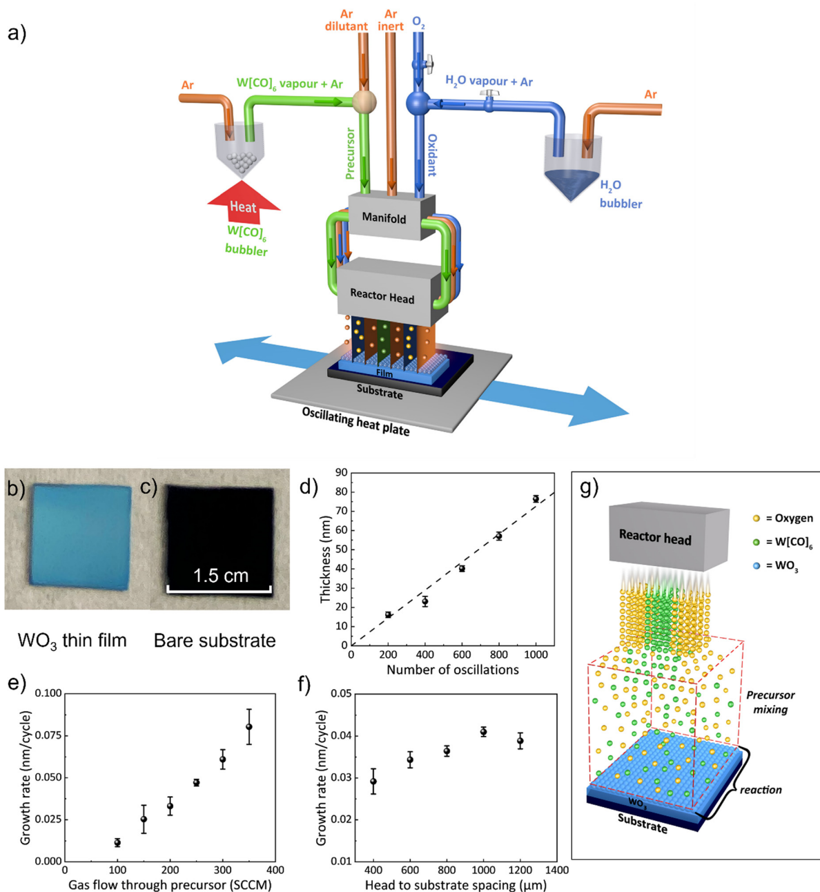
Fig. 1 Basic properties of WO 3 film growth using AP-SCVD. (a) Schematic of AP-SCVD system for the WO 3 film deposition, (b) optical image of WO 3 thin film grown on SiO 2 /Si substrate using O 2 as the oxidant, (c) bare SiO 2 /Si substrate, (d) thickness of WO 3 films on SiO 2 /Si substrate as a function of the number of substrate oscillations, (e) growth rate as a function of W[CO] 6 bubbler flowrate at a head-to-substrate spacing of 800 μm, (f) film growth rate as a function of head to substrate spacing at an Ar through precursor flowrate of 200 sccm, (g) schematic diagram showing how gas mixing occurs under the reactor head to give a CVD growth mode.
