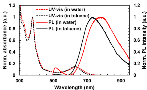
Fig. 3 (dotted line) UV-vis absorption and (real line) PL spectra of TTM-PEG3 in (red) water ( 10^{-5} M) and (black) toluene ( 10^{-5} M) for comparison.
