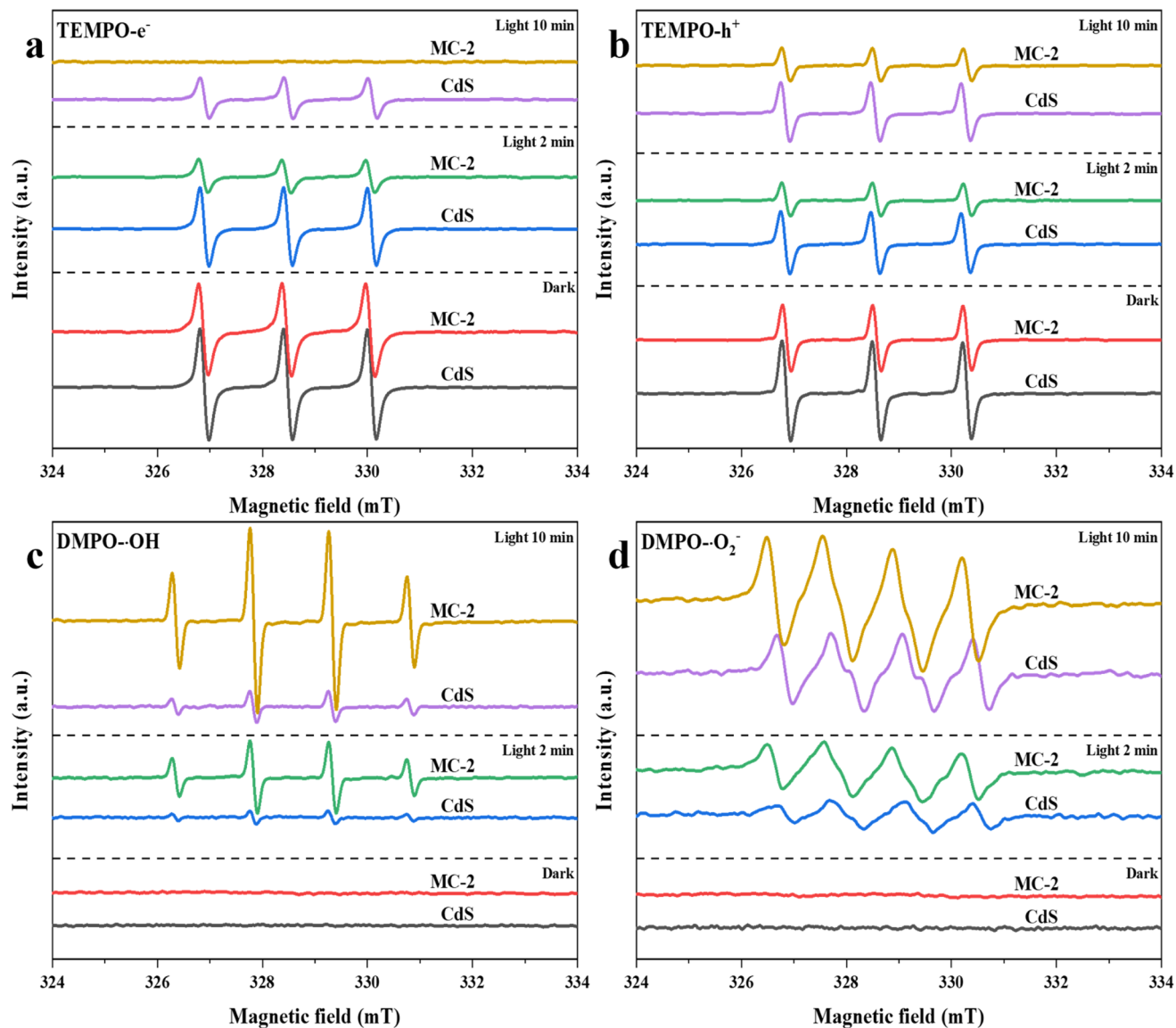
Fig. 7 ESR spectra of (a) TEMPO-e - , (b) TEMPO-h + , (c) DMPO- • OH, and (d) DMPO- • O 2 - adducts.
