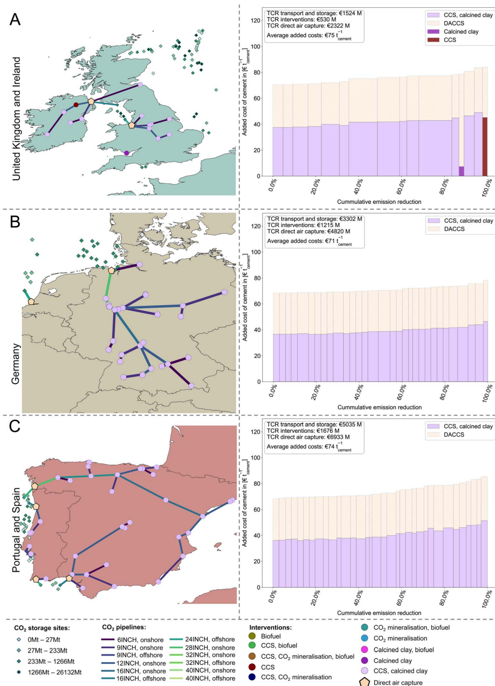
Fig. 4 Model results for reaching net-zero-CO 2e -emissions in (A) United Kingdom and Ireland, (B) Germany and (C) Portugal and Spain. Each circle represents one integrated cement plant and each orange pentagon a direct air capture location. Circle colours represent interventions. Line colours indicate CO 2 transport pipe thickness. Right panels show marginal CO 2e abatement cost curves for each region, each bar represents a single cement plant. Total capital requirements (TCR) describe the capital expenditures (CAPEX) of an investment. Assumptions and used calculations shown in Tables S6–S12, S14–S24.†
