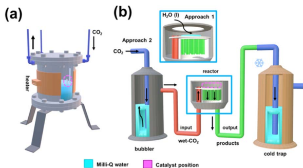
Scheme 2 (a) Scheme of the batch reactor used. (b) Scheme of the continuous reactor used. The continuous reactor was filled with four up-HAp catalysts ( 3.60 \times 5.00 \times 0.44 \text{ mm}^3 each) and 1 mL of deionized water which was homogeneously distributed (approach 1). The outlet valve of the reactor was connected to a cold trap to condense the reaction products obtained in the gas phase, while the inlet valve was connected to a \text{CO}_2 cylinder to achieve a constant flow of 100 \text{ mL s}^{-1} , which was controlled using a back-pressure regulator. This high flow was selected to mimic the conditions at the pre-pilot scale. To have the required moisture, as water is the proton source, \text{CO}_2 was bubbled into liquid water to produce wet \text{CO}_2 , the bubbler being located between the \text{CO}_2 cylinder and the inlet valve (approach 2).
