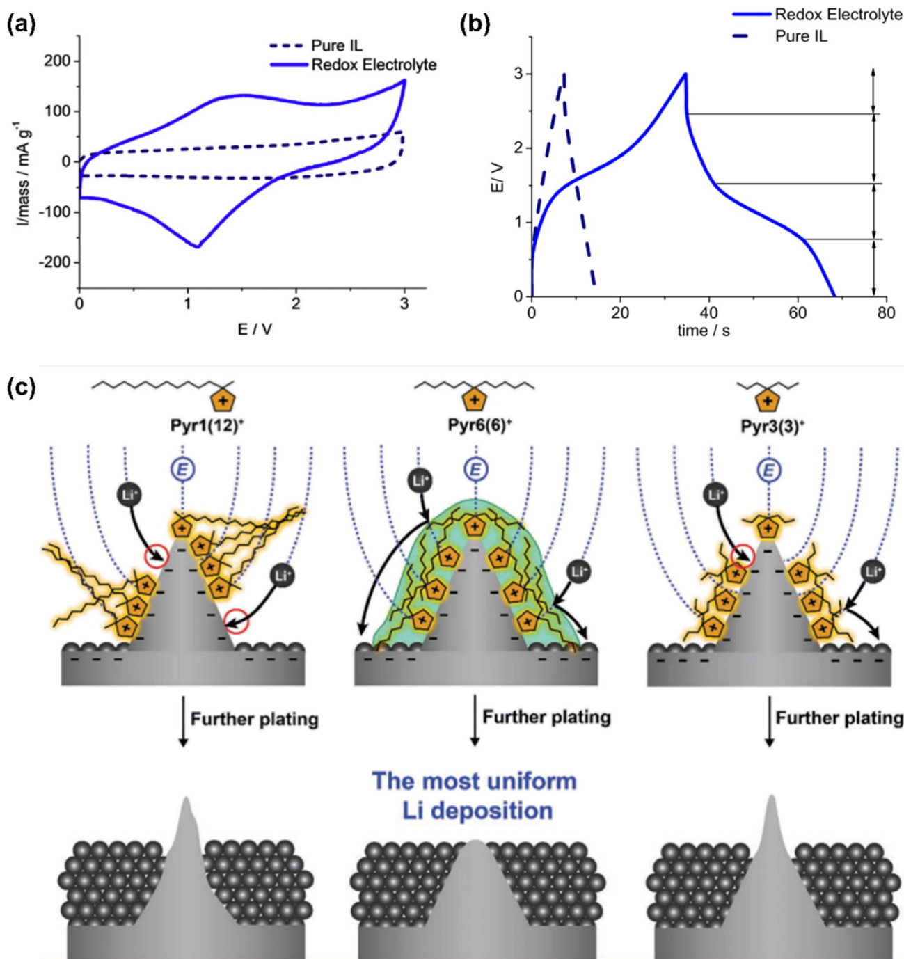
Fig. 8 (a) Cyclic voltammograms and (b) galvanostatic charging and discharging profiles up to 3.0 V of a symmetrical cell of Vulcan carbon. Electrolytes: redox IL electrolyte of 0.4 M p -BQ in \text{PYR}_{14}\text{TFSI} (solid blue lines) and pure \text{PYR}_{14}\text{TFSI} (dashed black lines). Temperature: 60 °C. Current density: 10 \text{mA cm}^{-2} . 33 (c) The impact of three different IL cations, \text{Pyr}_1(12)^+ (left), \text{Pyr}_6(6)^+ (middle), and \text{Pyr}_3(3)^+ (right), on inducing uniform Li metal deposition owing to the formation of lithiophobic protective layers on Li protuberances. 99 (Reprinted from ref. 33 and 99 with permission from Rightslink).
