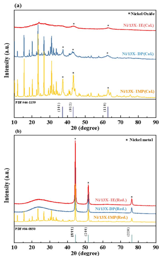
Fig. 2 XRD patterns of (a) calcined and (b) reduced Ni/zeolite 13X catalysts.
