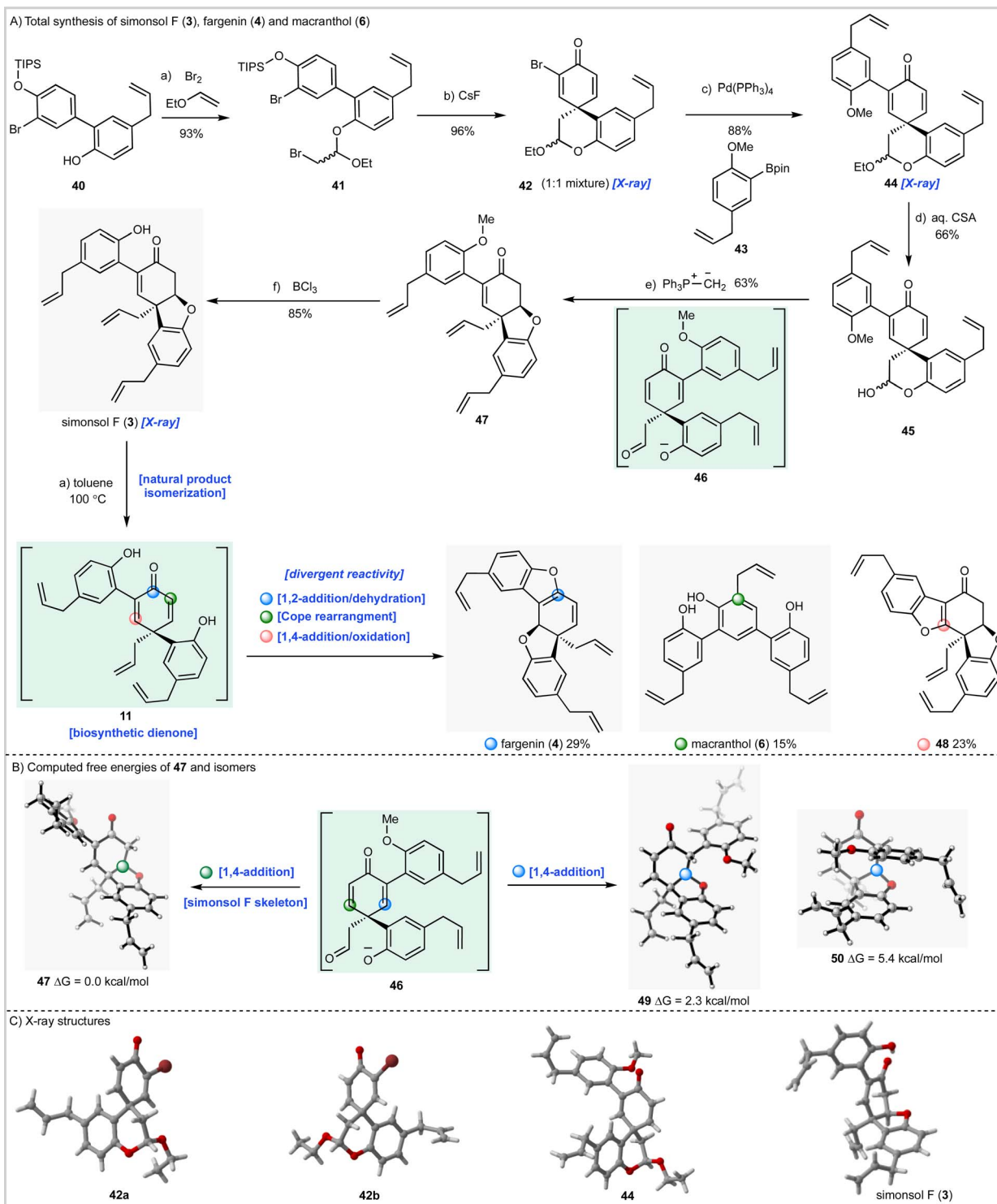
Scheme 3 Total synthesis of simonsol F ( 3 ) and its possible biomimetic conversion into fargenin ( 4 ) and macranthol ( 6 ). (A) Reagents and conditions: (a) ethyl vinyl ether, \text{Br}_2 , Hünig's base, DCM, 0^\circ\text{C} to r.t., 2.5 h, 93%; (b) CsF, \text{Na}_2\text{SO}_4 , DMF, 130^\circ\text{C} , 1 h, 96%; (c) \text{Pd}(\text{PPh}_3)_4 , aq. \text{Na}_2\text{CO}_3 , toluene:ethanol, 85^\circ\text{C} , 4 h, 88%; (d) CSA, \text{H}_2\text{O} , 1,4-dioxane, 85^\circ\text{C} , 10.5 h, 66%; (e) \text{MePPh}_3\text{Br} , KHMDs, THF, 0^\circ\text{C} , 0.5 h, 63%; (f) \text{BCl}_3 , DCM, 0^\circ\text{C} , 5.5 h, 85%; (a) toluene- d_8 , 100^\circ\text{C} , 228 h, macranthol ( 6 ) 15%, fargenin ( 4 ) 29%, 58 23%. (B) Computed free energies of 47 and isomers. (C) X-ray structures. DCM = dichloromethane, CSA = camphorsulfonic acid.
