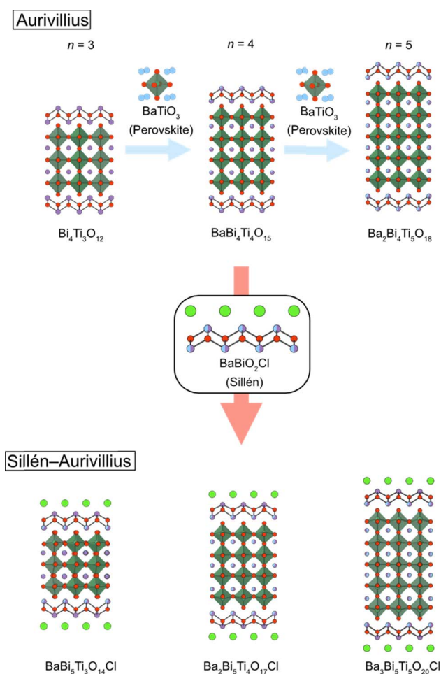
Fig. 15 An illustration of the bricklaying synthesis for multi-layered Sillén–Aurivillius phases \text{BaBi}_5\text{Ti}_3\text{O}_{14}\text{Cl} ( n = 3 ), \text{Ba}_2\text{Bi}_5\text{Ti}_4\text{O}_{17}\text{Cl} ( n = 4 ) and \text{Ba}_3\text{Bi}_5\text{Ti}_5\text{O}_{20}\text{Cl} ( n = 5 ). 38
