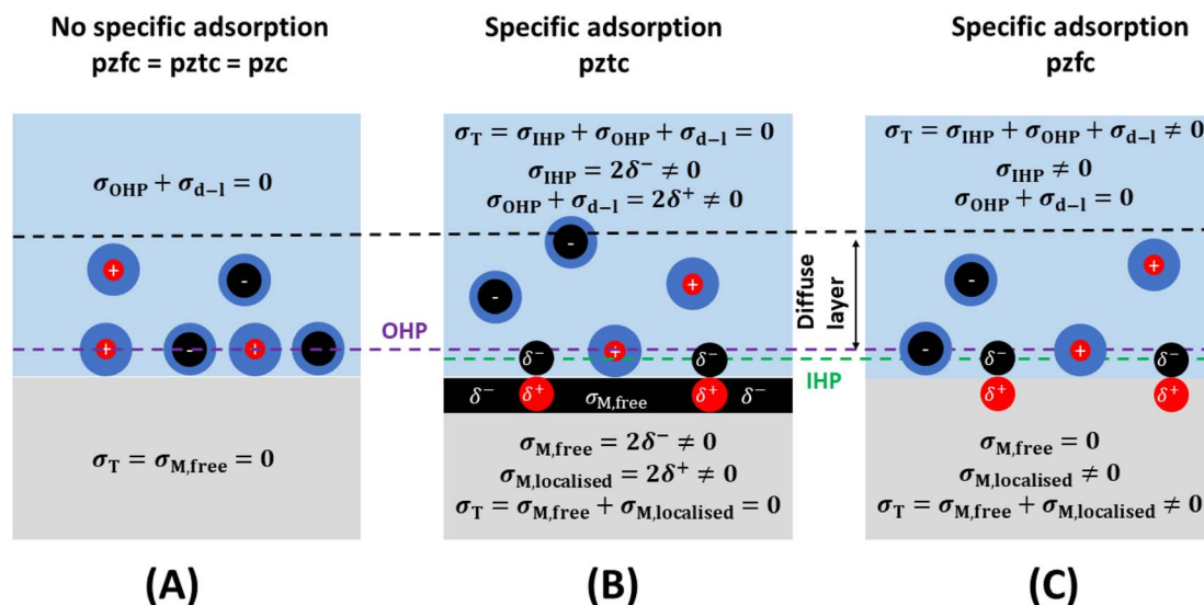
Fig. 3 The pzfc and the pztc . In the absence of specific adsorption (A), the pztc and the pzfc coincide. When there are specifically adsorbed species on the metal surface (B and C), the free charge density on the metal surface is not zero at the pztc (B), while the total charge density is not zero at the pzfc (C).
