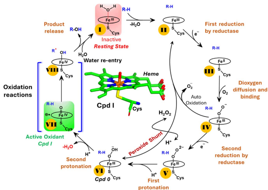
Scheme 1 A generic catalytic cycle for CYP450 enzymes using \text{O}_2 , 2e^- , and \text{H}^+ (steps: I \rightarrow II \rightarrow III \rightarrow IV \rightarrow V \rightarrow VI \rightarrow VII) and using directly \text{H}_2\text{O}_2 (peroxide shunt) as a co-substrate to generate the active oxidant Cpd I by the CYP450 peroxxygenase family.
