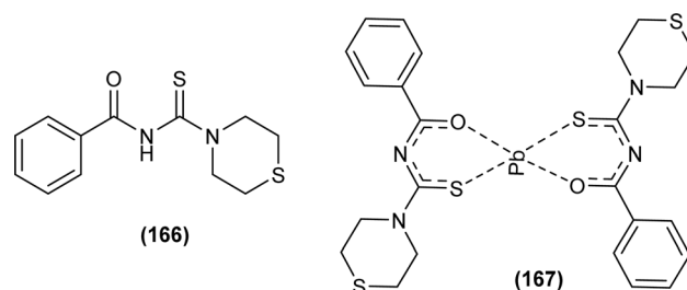
Fig. 92 N -(Thiomorpholine-4-carbothiyl)benzamide and its Pb(ii) complex.
