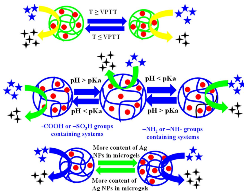
Fig. 7 Different catalytic reaction affecting factors (reproduced from ref. 11 with permission from Elsevier, copyright 2023). 11
