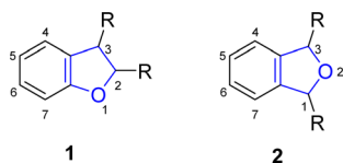
Fig. 1 General structure of dihydrobenzofuran 1 and dihydroisobenzofuran 2 .
